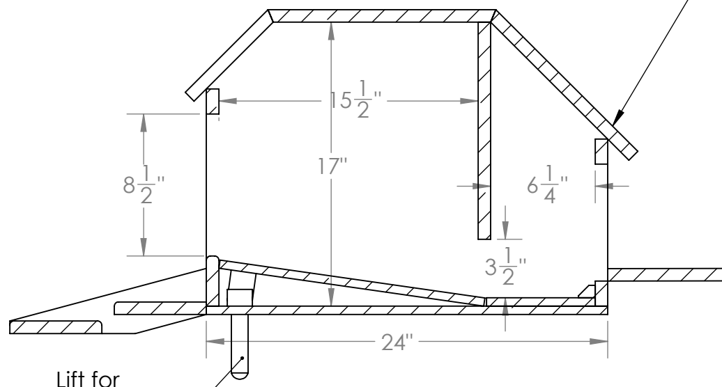
Roll Out Nest Box Mk3
