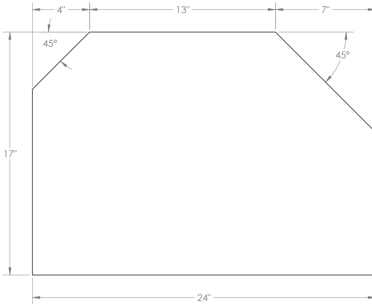
RONB Mk3 Side Material 3/4" Plywood
