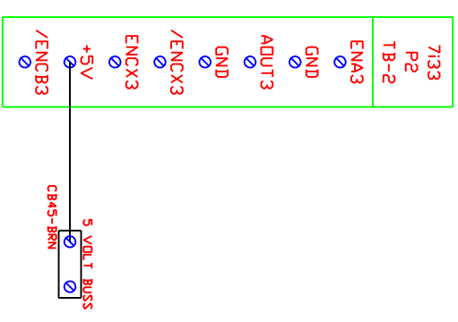
1 24vdc 3 0vdc 7133 Quad Servo Card TB-2
