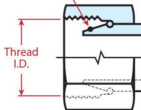
24° Taper with O-Ring
