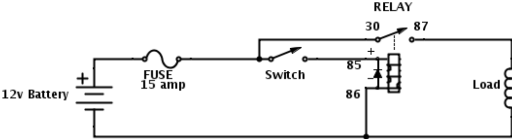
Connection Diagram
